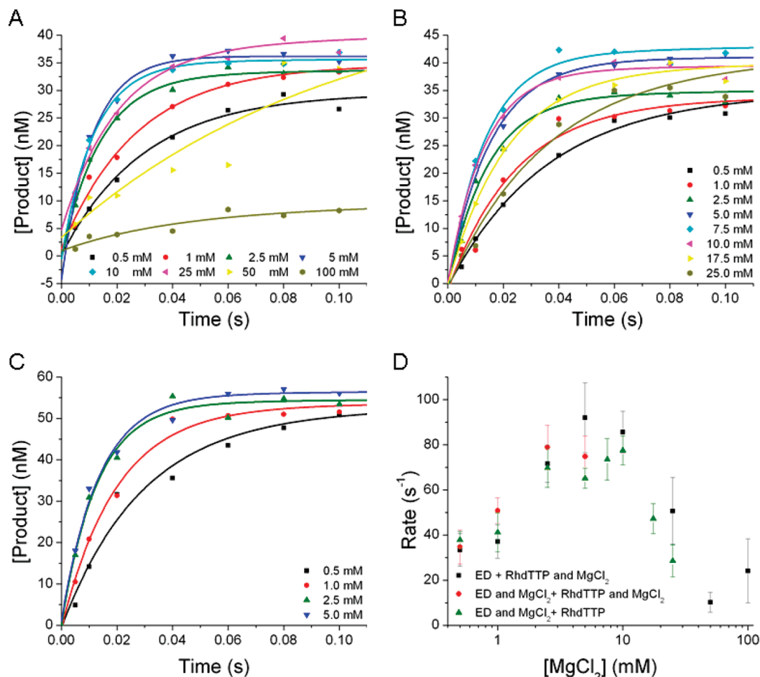
FIGURE 1: Incorporation of Rh•dTTP opposite dA at varying concentrations of MgCl 2 . The final reaction conditions for all experiments depicted consisted of 100 nM RB69 pol, 90 nM DNA, 250 \mu M Rh•dTTP, 50 mM MOPS (pH 7.0), and varying concentrations of MgCl 2 from 0.5 to 100 mM. (A) The reaction was initiated by premixing Rh•dTTP and MgCl 2 and then rapidly mixing this solution with one containing RB69 pol and DNA. The incorporation rate is 92 \pm 15 \text{ s}^{-1} . (B) The reaction was initiated by premixing RB69 pol, DNA, and MgCl 2 and then rapidly mixing this solution with one containing Rh•dTTP. The incorporation rate is 77 \pm 6 \text{ s}^{-1} . (C) The reaction was initiated by premixing RB69 pol, DNA, and MgCl 2 and then rapidly mixing this solution with one containing Rh•dTTP and MgCl 2 . The incorporation rate is 80 \pm 10 \text{ s}^{-1} . (D) The rates of product formation are plotted vs MgCl 2 concentration for each of the three experiments depicted in panels A–C. Regardless of when MgCl 2 is added, the observed maximum rate of the reaction fits to approximately 80 \text{ s}^{-1} , at a MgCl 2 concentration of approximately 10 mM. Because of the mixing procedure, each solution was prepared at twice the final reported concentration. The product concentrations were plotted vs time and fit to a single-exponential equation.
