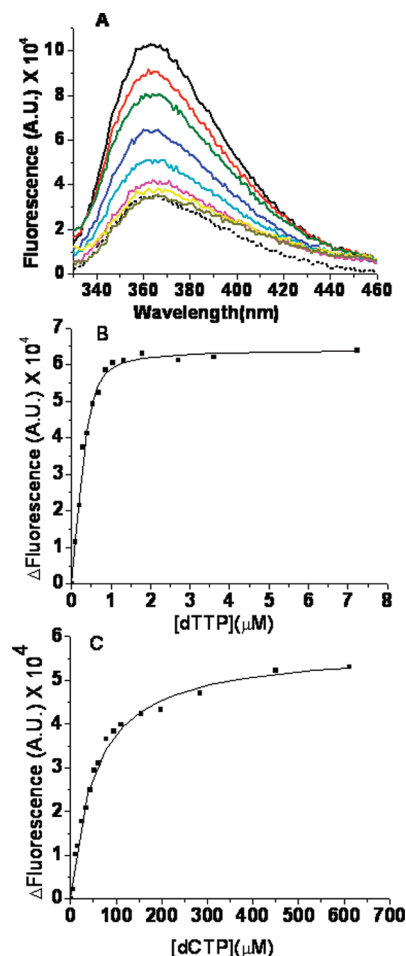
FIGURE 3: Equilibrium fluorescence titrations for dTTP or dCTP binding to the RB69 DNA pol–dP/T complex. (A) Representative fluorescence emission spectra of dTTP binding to wild-type RB69 pol in the presence of a 13/20mer dP/T (Table 1), with dAP as the templating base (shown by the solid lines) and 2 mM \text{CaCl}_2 . The concentration of dP/T was 200 nM, and that of RB69 pol was 1 \mu\text{M} . The dTTP concentrations (from top to bottom) were 0, 0.1, 0.2, 0.3, 0.55, 0.9, 2.9, and 7.9 \mu\text{M} . The dotted line is the fluorescence trace for the dP/T alone. (B) dP/T (dAP as the templating base, 200 nM) in the presence of 2 mM \text{Ca}^{2+} . The change in fluorescence vs dTTP concentration fit best to a quadratic binding equation with a K_{\text{dg}}^{\text{app}} of 0.053 \pm 0.015 \mu\text{M} . (C) dP/T (dAP as the templating base, 200 nM). The change in fluorescence vs dCTP concentration fit best to a hyperbolic equation with a K_{\text{dg}}^{\text{app}} of 53 \pm 3 \mu\text{M} . The change in fluorescence ( \Delta F ) is in the direction of quenching. The \Delta F of the binary complex is normalized to zero in the absence of dNTP, and the \Delta F increases with an increase in dNTP concentration.
