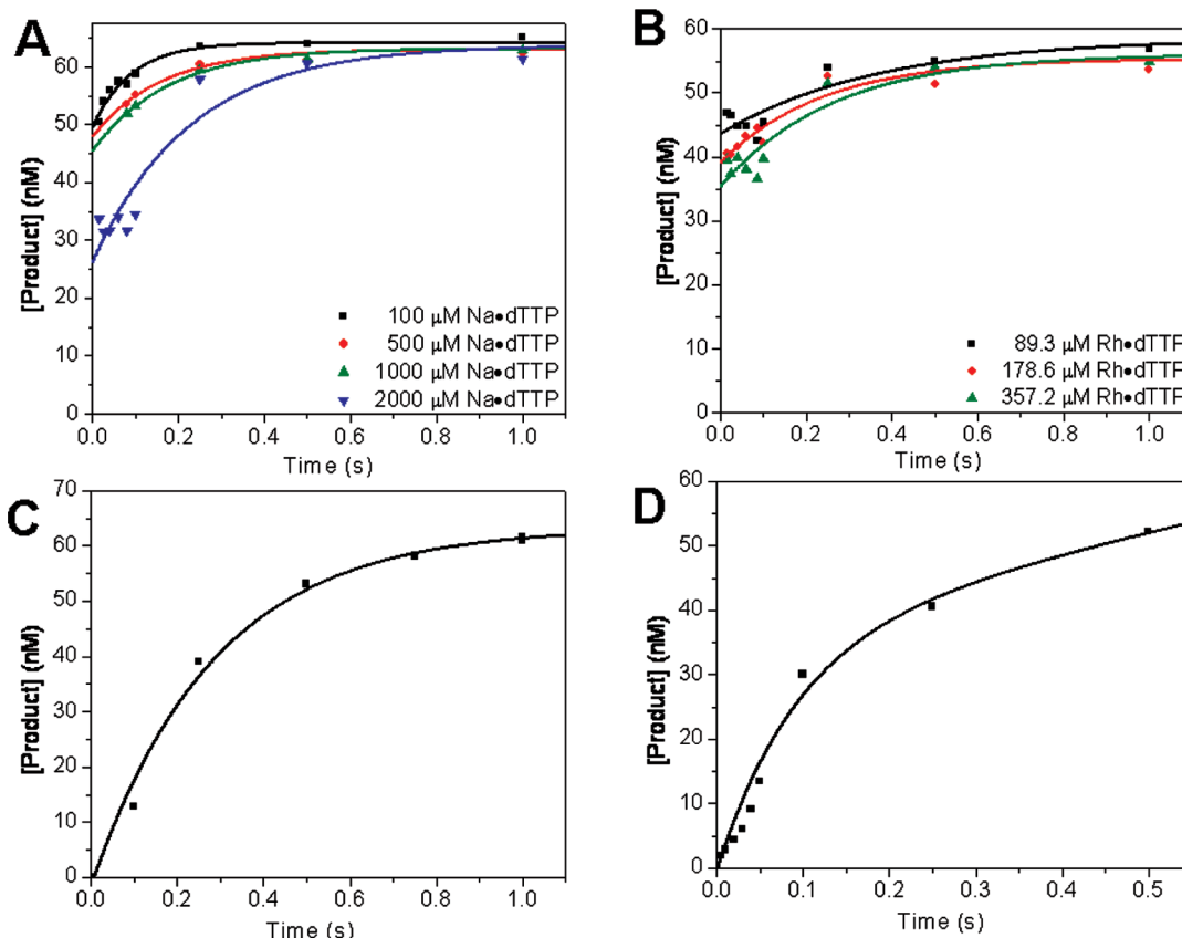
FIGURE 2: Pulse-chase, chemical-quench experiment. (A) RB69 pol was preincubated with DNA, then rapidly mixed with various Na•dTTP concentrations, and allowed to incubate for 0.01 s. (B) RB69 pol was preincubated with DNA, then rapidly mixed with various Rh•dTTP concentrations, and allowed to incubate for 0.01 s. (C) RB69 pol was preincubated with DNA, then rapidly mixed with 500 \mu M dTTP and 4 mM \text{CaCl}_2 , and allowed to incubate for 0.01 s. After preincubation, each reaction mixture was rapidly mixed with \text{MgCl}_2 and allowed to react for variable amounts of time before the reaction was quenched with 0.5 M EDTA. The data from panels A–C were fit to a single-exponential equation, and the average rates are 8 \pm 4 , 4 \pm 1 , and 3.5 \pm 0.4 \text{ s}^{-1} , respectively. (D) dTTP (500 \mu M) was preincubated with 4 mM \text{CaCl}_2 and 10 mM \text{MgCl}_2 and then rapidly mixed with a solution containing RB69 pol, DNA, and 10 mM \text{MgCl}_2 . The reaction was quenched at various times with 0.5 M EDTA, and the data were fit to a burst equation. The burst rate is 11 \pm 4 \text{ s}^{-1} . The final reaction conditions included 100 nM RB69 pol, 90 nM DNA, 50 mM MOPS (pH 7.0), and 10 mM \text{MgCl}_2 .
