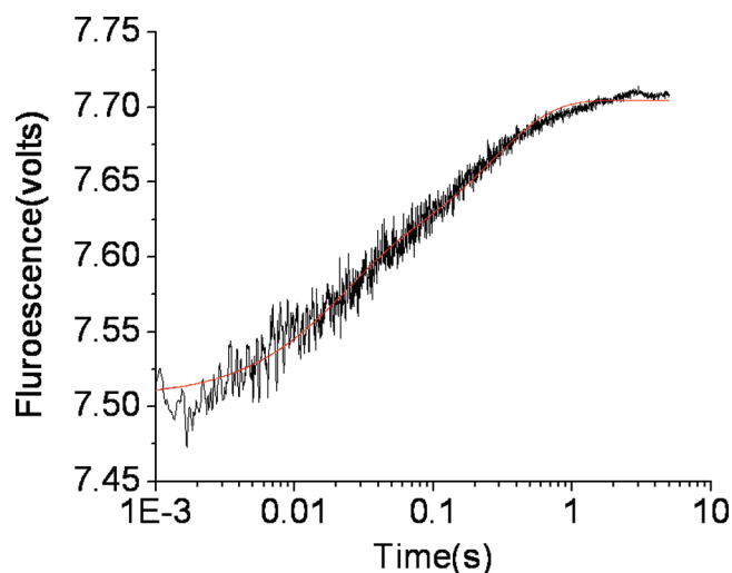
FIGURE 6: Sq-dP/T + binary complex trapping of dTTP released from a RB69 pol-dP/T*-dTTP ternary complex using stopped-flow fluorescence with dTTP opposite dAP with a dP/T (Table 1). The fluorescence vs time fit best to a double-exponential equation with rates of 50 and 4 s -1 .
