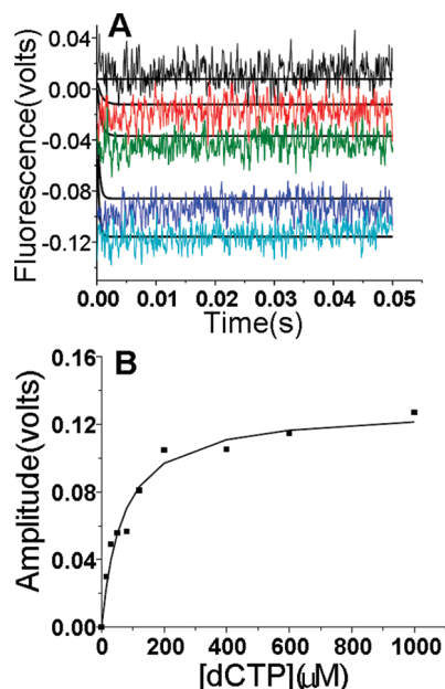
FIGURE 5: Stopped-flow fluorescence scans with dCTP opposite dAP with a dP/T. (A) One syringe contained 400 nM DNA and 2 μM RB69 pol in 50 mM MOPS buffer (pH 7) at 24 °C. The other syringe contained varying dCTP concentrations (0, 15, 50, 400, and 1000 μM from top to bottom) in MOPS buffer. Both syringes contained 2 mM CaCl 2 . The fitting plot was obtained from the estimated parameters based on Scheme 2. The experimental scans are in color, and the fitting curves are in black. (B) The amplitude vs dCTP concentration fit a hyperbolic equation with a K_{da}^{app} of 67 \pm 12 μM.
